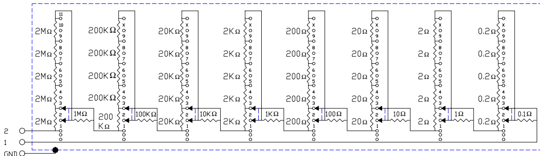
Figure 2 Model DB877 Schematic
